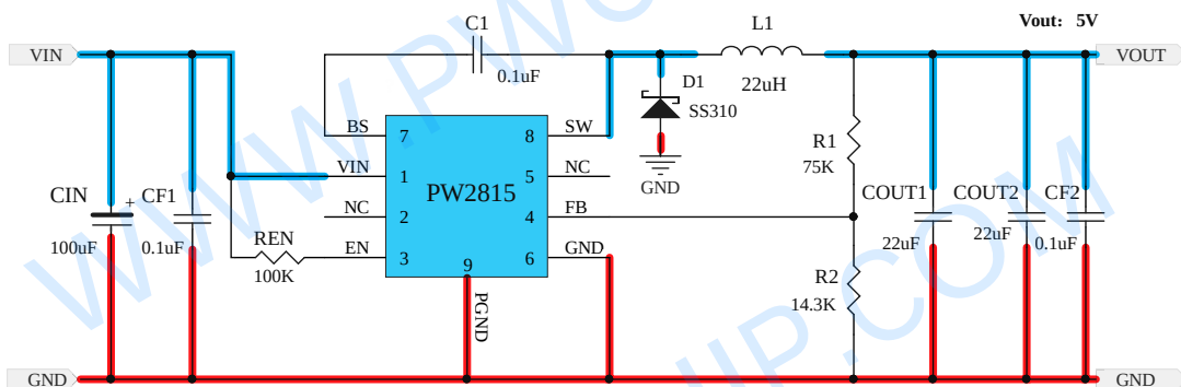
PW2815_DEMO_Typical Circuit:
