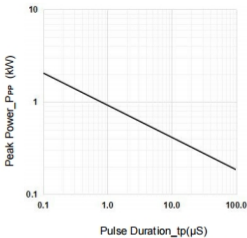
Peak Pulse Power vs. Pulse Time
