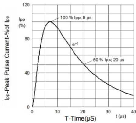
IEC61000-4-5 8X20 \mu\text{s} Pulse Waveform
